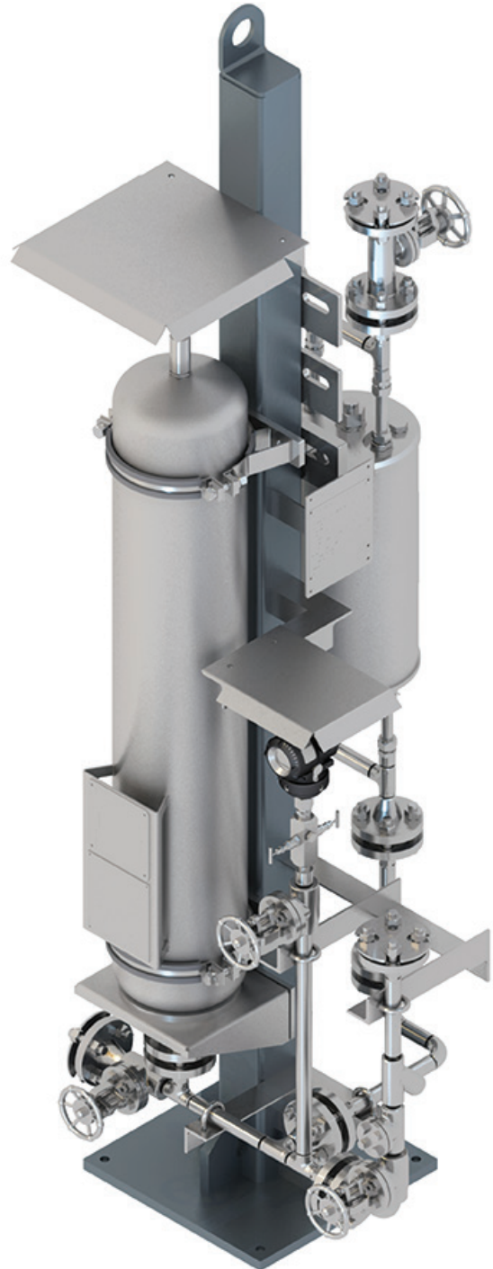
Flowserve 682-53B seal support system with 682H Seal Cooler
