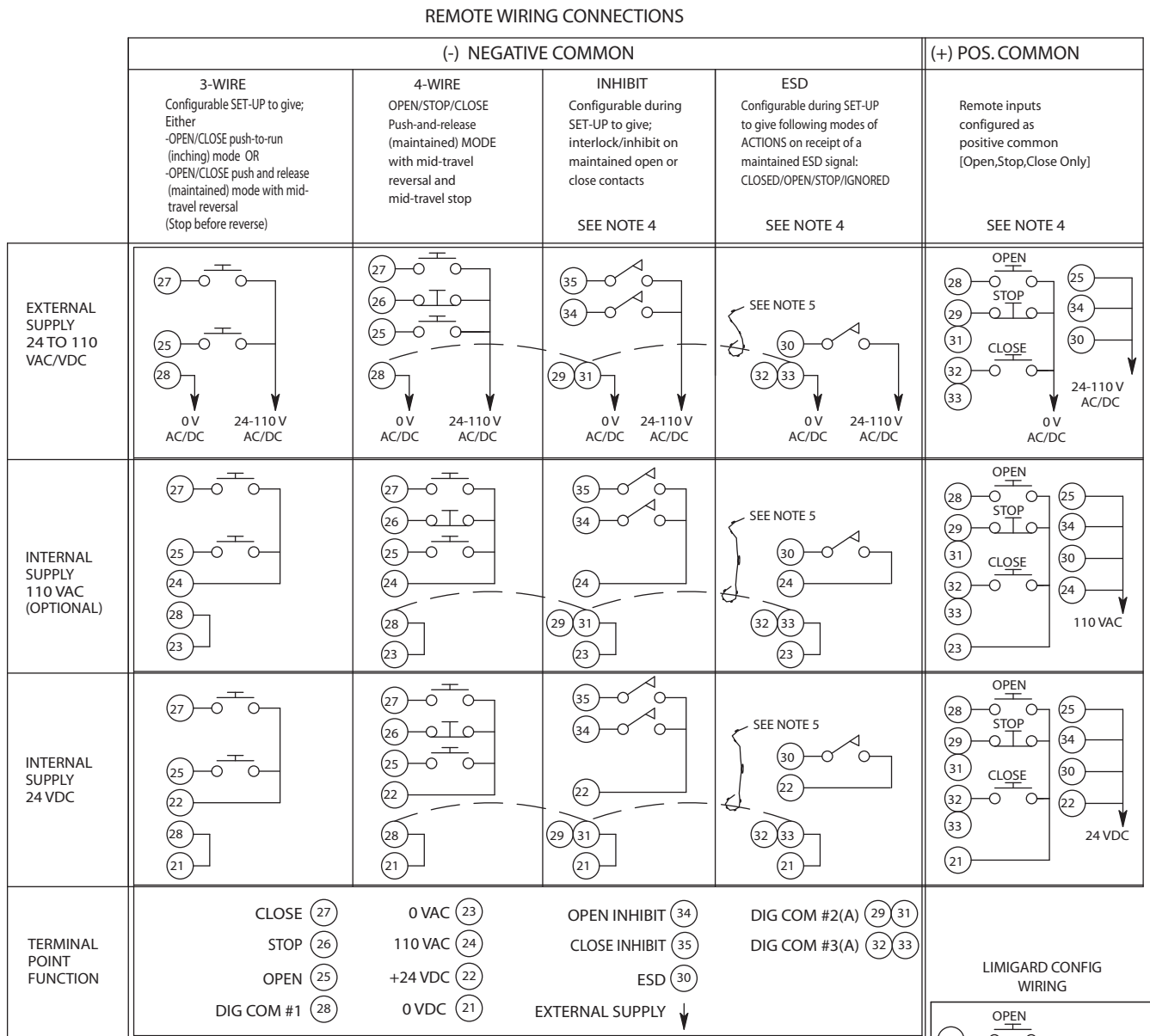
Figure 13.5 – Remote Wiring Connections
