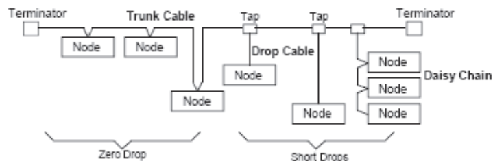
Figure 14.5 – Typical DeviceNet Network
