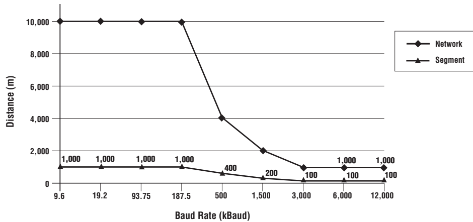
Figure 14.4 – PROFIBUS Distance vs. Baud Rate Chart
