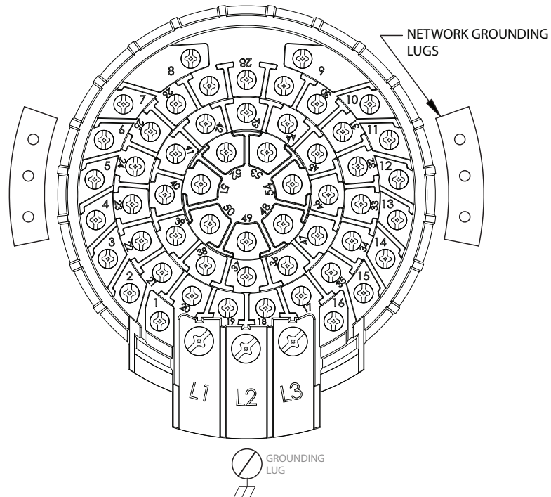
Figure – 12.1 MX/QX terminal block
