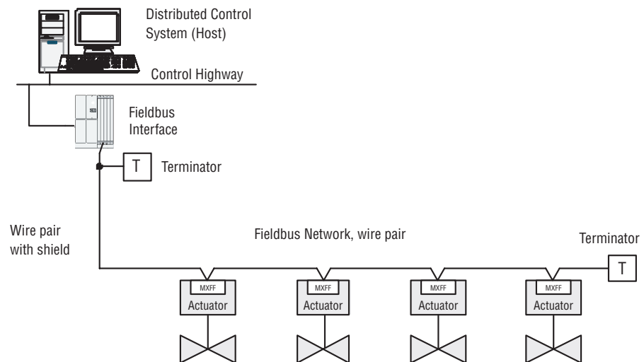
Figure 14.2 – Typical Foundation Fieldbus Network With DCS or PLC as the Host System
